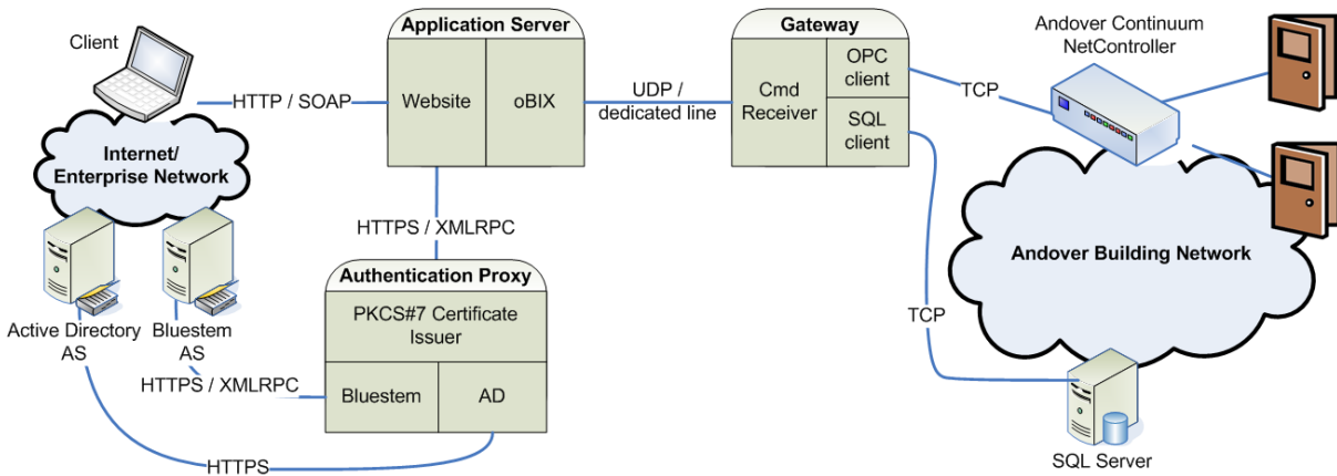
Figure 4: Prototype Architecture
