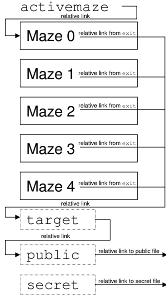
Figure 9: Malicious directory structure for attacking the randomized k -Race defense. The exit links in each maze point to the symbolic link target and the attacker points target to the public or protected file depending on the victim’s current system call.
